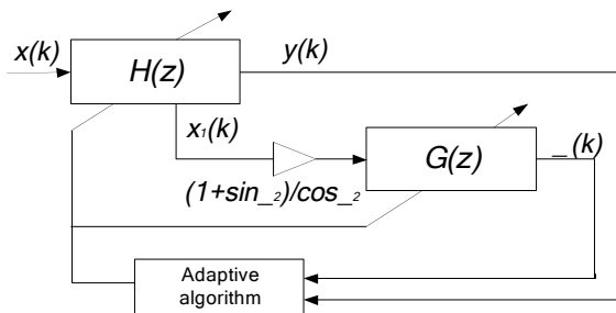
Fig. (2). Design diagram of adaptive cascade notch filter.
