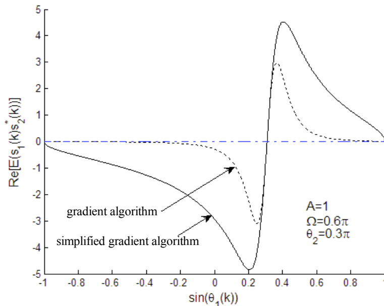
Fig. (3). Output response function of the adaptive cascade notch filter in cyber-attack model.
