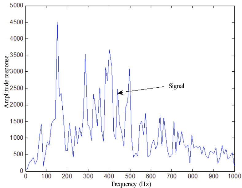
Fig. (5). Output of preprocessing by the adaptive cascade notch filter.
