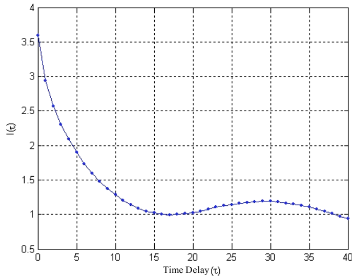
Fig. (1). Curve of delay parameter variation in Rossle chaotic system.
